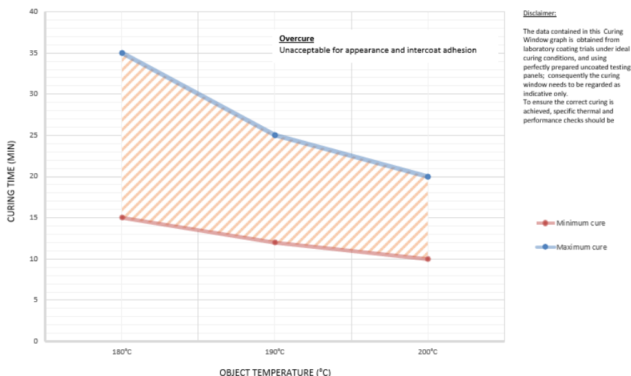
Interpon D2525 Structura - curing window
